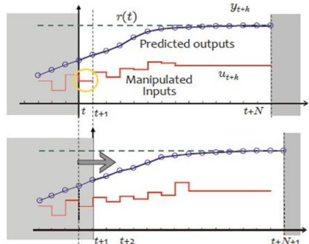
Figure 8 Moving horizon approach of MPC
