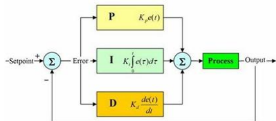
Figure 7 PID Controller
