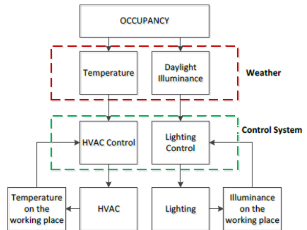
Figure 5 Proposed Control Strategy
