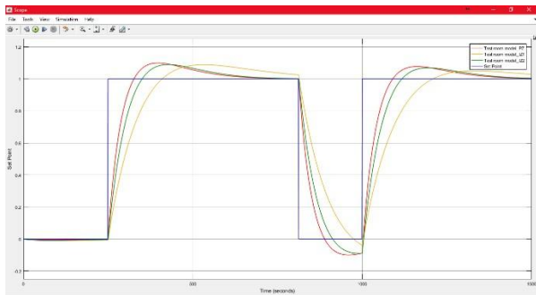
Figure 10 Simulation result using PID Controller
