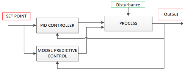
Figure 6 HVAC control scheme
