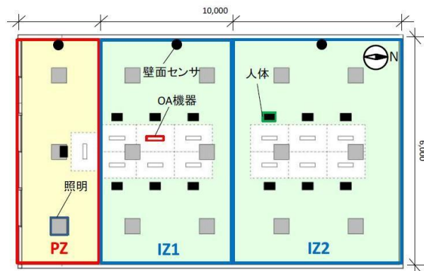
Figure 4 Room Layout
