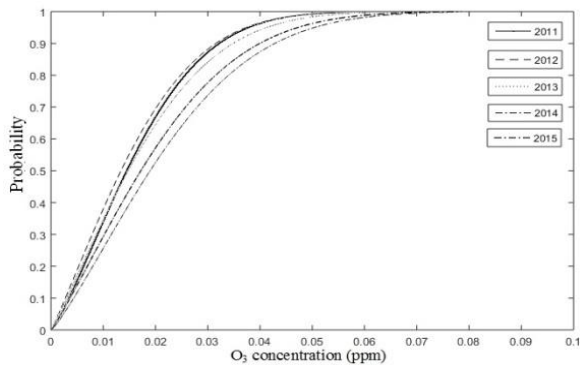
Fig. 4 Cumulative distribution function (CDF) of ground level ozone for Kuala Terengganu.
