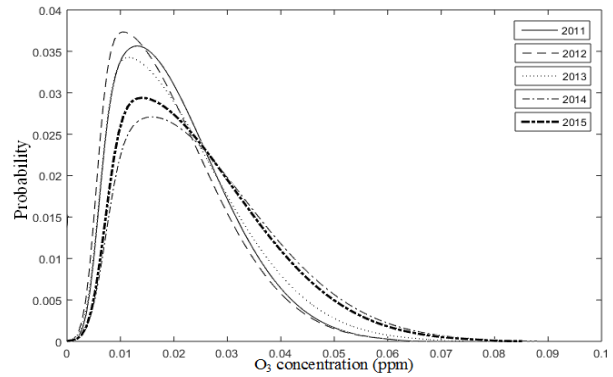
Fig. 1 Probability density function (PDF) plot of ground level ozone for Kuala Terengganu.
