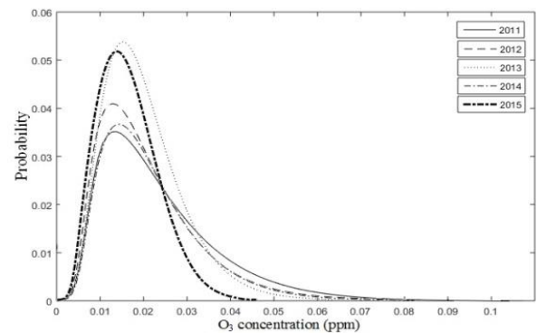
Fig. 3 Probability density function (PDF) plot of ground level ozone for Alor Setar.
