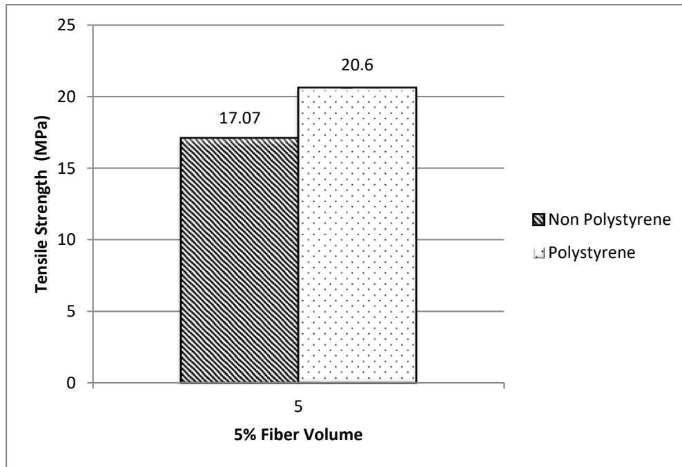
Fig. 2 Effect of 5% volume into coconut meat husk fiber reinforced Polyester
